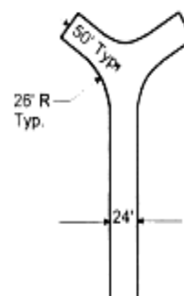
Fig. 4 ACCEPTABLE ALTERNATIVE TO 100' HAMMERHEAD
