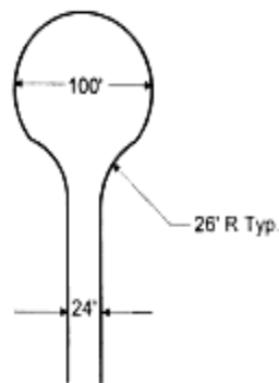
Fig. 1 100' DIAMETER CUL-DE-SAC
