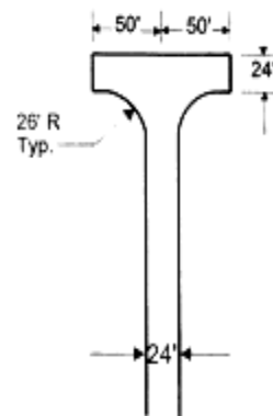
Fig. 2 100' HAMMERHEAD
