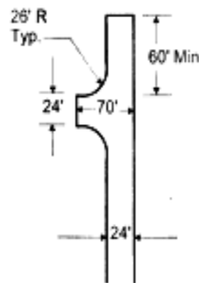
Fig. 3 ACCEPTABLE ALTERNATIVE TO 100' HAMMERHEAD
