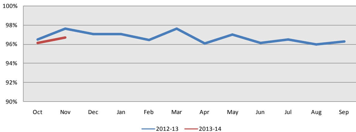
Uptime Percentage
